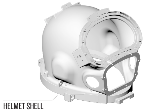
Blowpart drawing of the handle and helmet shell.
