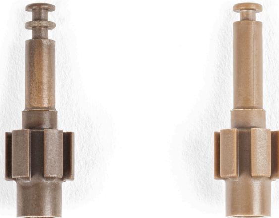
Previous balance spacer with two O-ring slots, left, and current with one, right.
