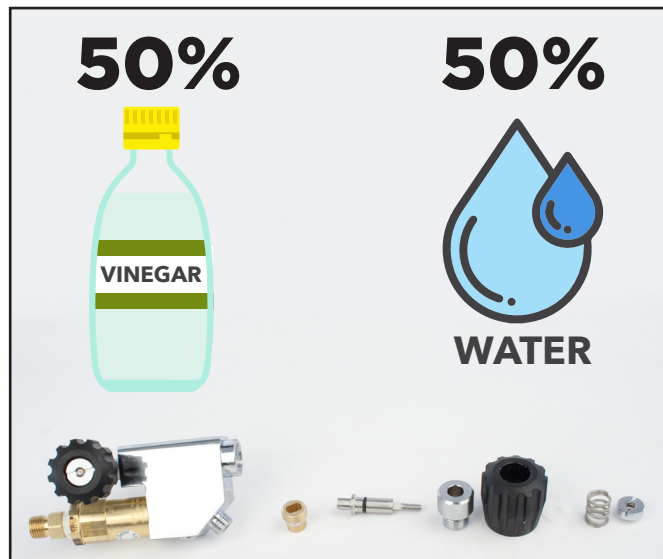
Clean all the metal parts to remove salts.
