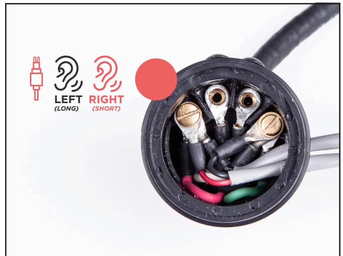
8. Insert the microphone wires into the module.
