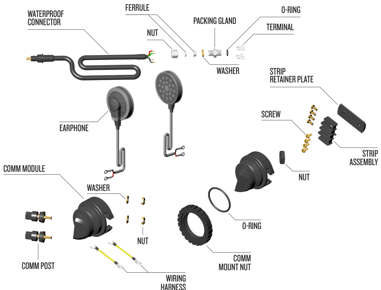
Components of the communications system (new design).
