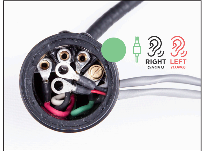
7. Using the washer and screw, install the black wire from the left ( long ) earphone and the red wire from the right ( short ) earphone.
