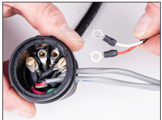
9. Using the washer and screw, install the red and white microphone wires to the module.
