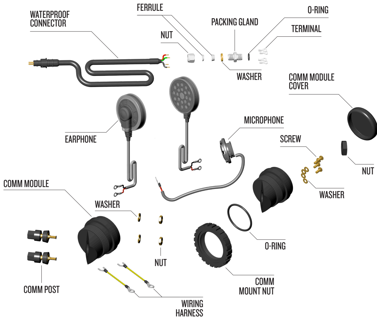
Components of the communications system (old design). See diagram "Components of the communications system (new design)." on page COM-15 for current design.
