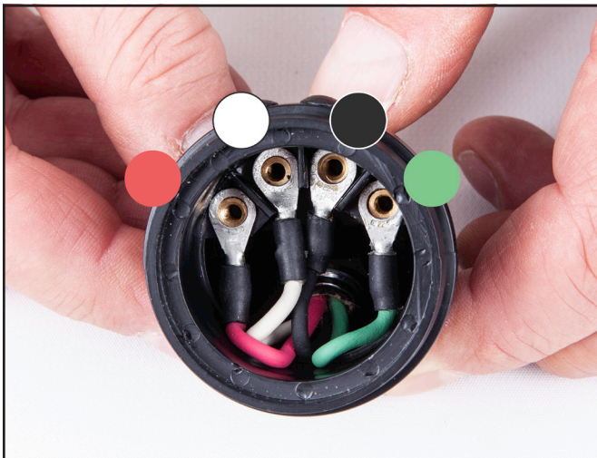
5. Insert the earphone wires back into the module.
