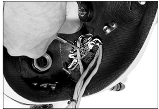
The terminal block is where you will disconnect the earphones from the helmet or mask.
