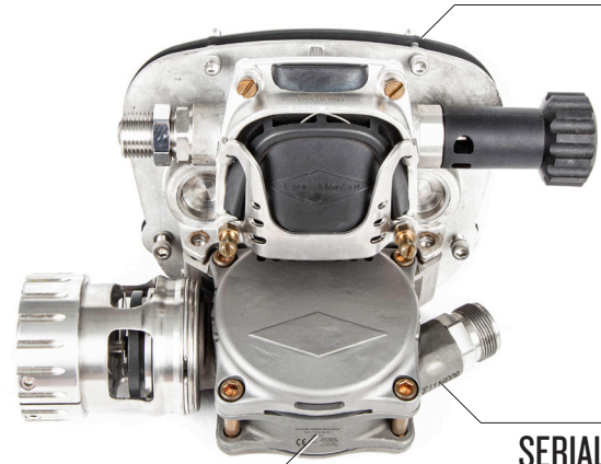
DIAMOND EXHAUST REGULATOR YEAR OF PRODUCTION: 2022 EN15333-1
