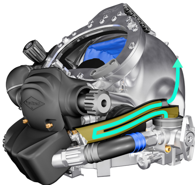
Sectional View of the Bypass Equalizer Tube in the Open Circuit Position
