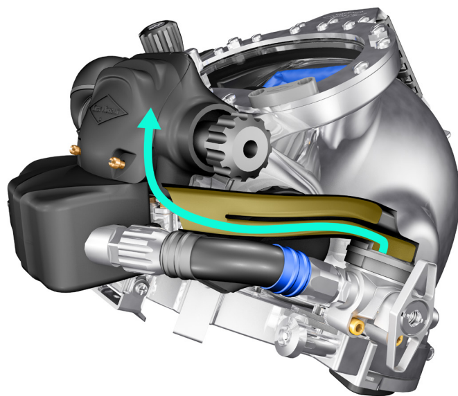
Sectional View of the Bypass Equalizer Tube in the Open Circuit Position
