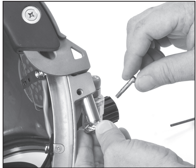
The screws that secure the sealed pulled pins must be properly installed and tightened.
