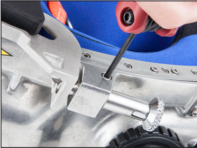
Unscrew the hex head bolts.
