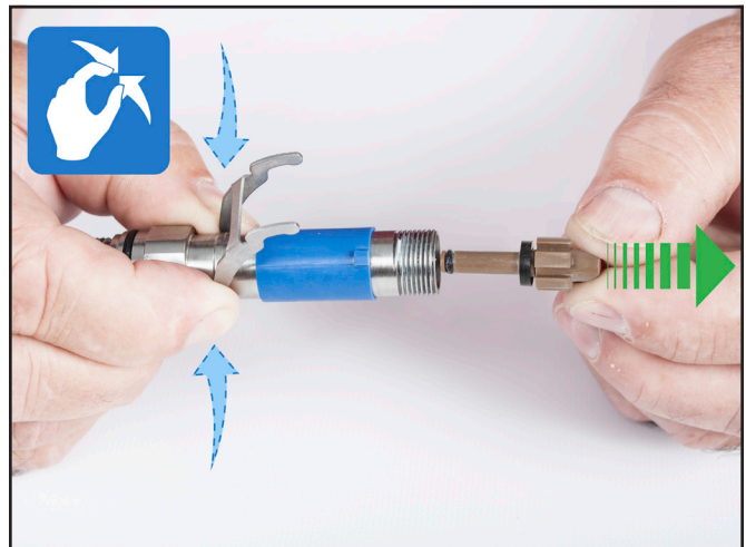
Pinch both sides of the lever arm against the main tube, and at the same time, remove the balance spacer with O-ring.
