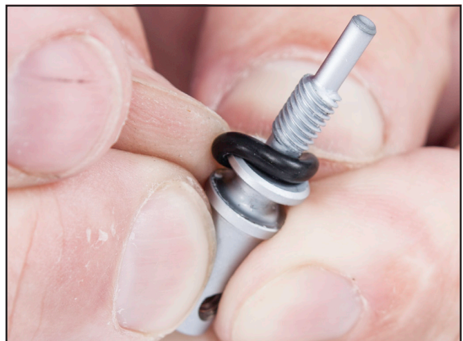
Lubricate O-ring and install onto the adjustment shaft.
