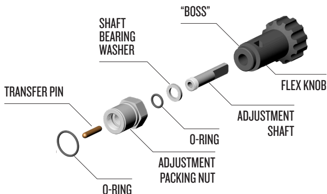
SuperFlow® 450 flex knob assembly.
