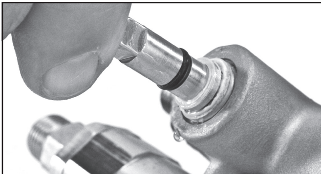
Install the new seat assembly using the stem.
