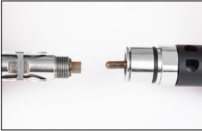
The transfer pin may fall from the end of the shaft. Be careful not to lose it.
