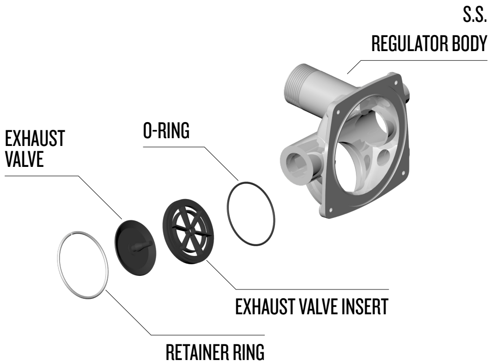
455 Balanced exhaust valve mechanism.
