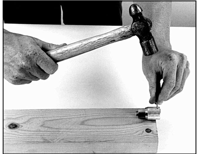
Install the retaining pin into the adjustment knob.
