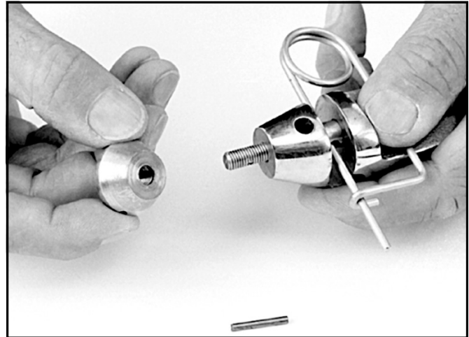
Once the pin is driven out, you can remove the knob from the plunger.
