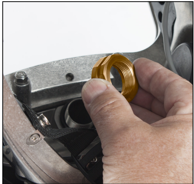
Install the regulator mount nut. DO NOT FULLY TIGHTEN THE NUT AT THIS TIME.
