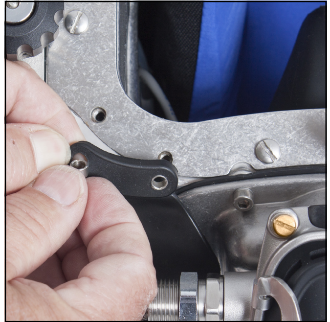
Attach the whisker to each side of the face port retainer using the spacers, zinc anodes or kidney plates and screws.
