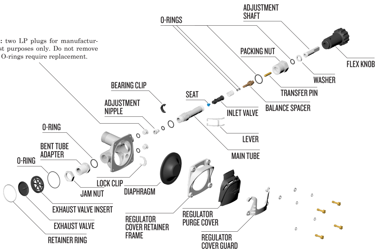
Exploded view of 455 Balanced regulator.
