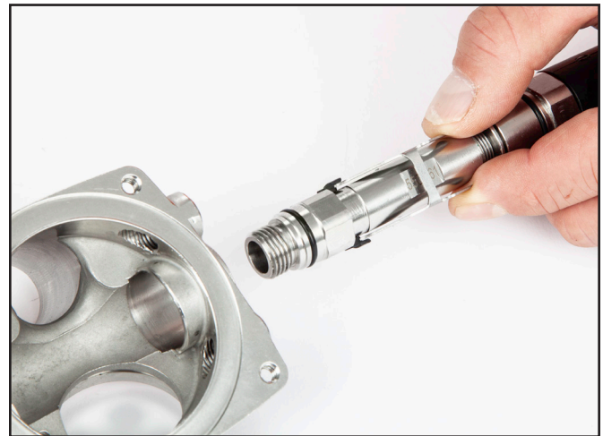
Depress the lever arm down and carefully install the main tube assembly into the regulator body.
