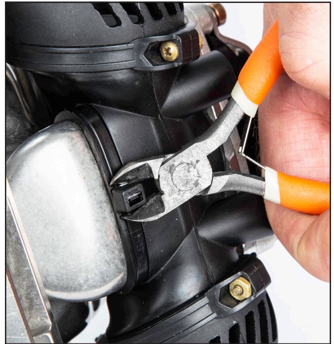
Cut the tie wrap that connects the quad valve exhaust main body to the water dump tube on the helmet pod.
