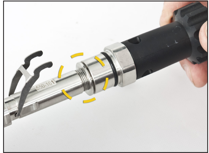
When installing the main tube into the regulator body it is critical to leave three plus threads exposed on the main tube.
