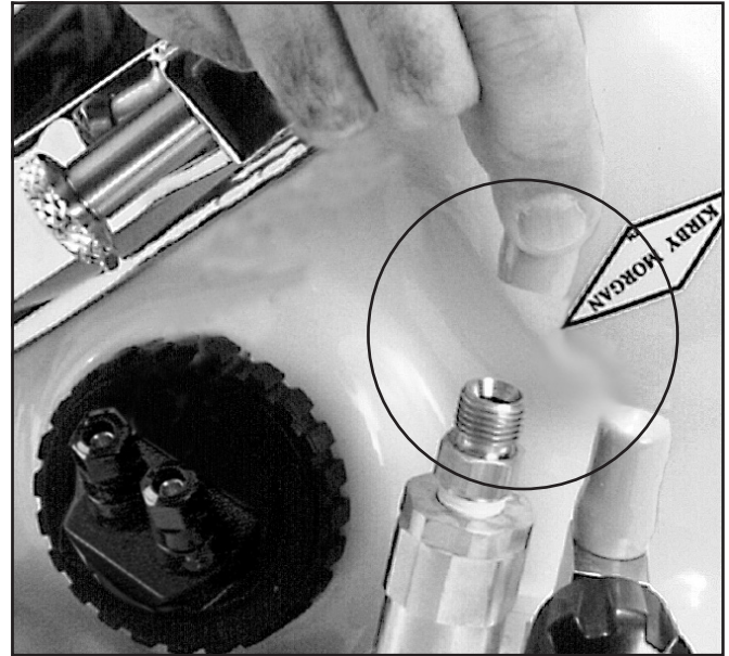
Cover the air inlet and emergency gas valve openings with dust caps when not in use.
